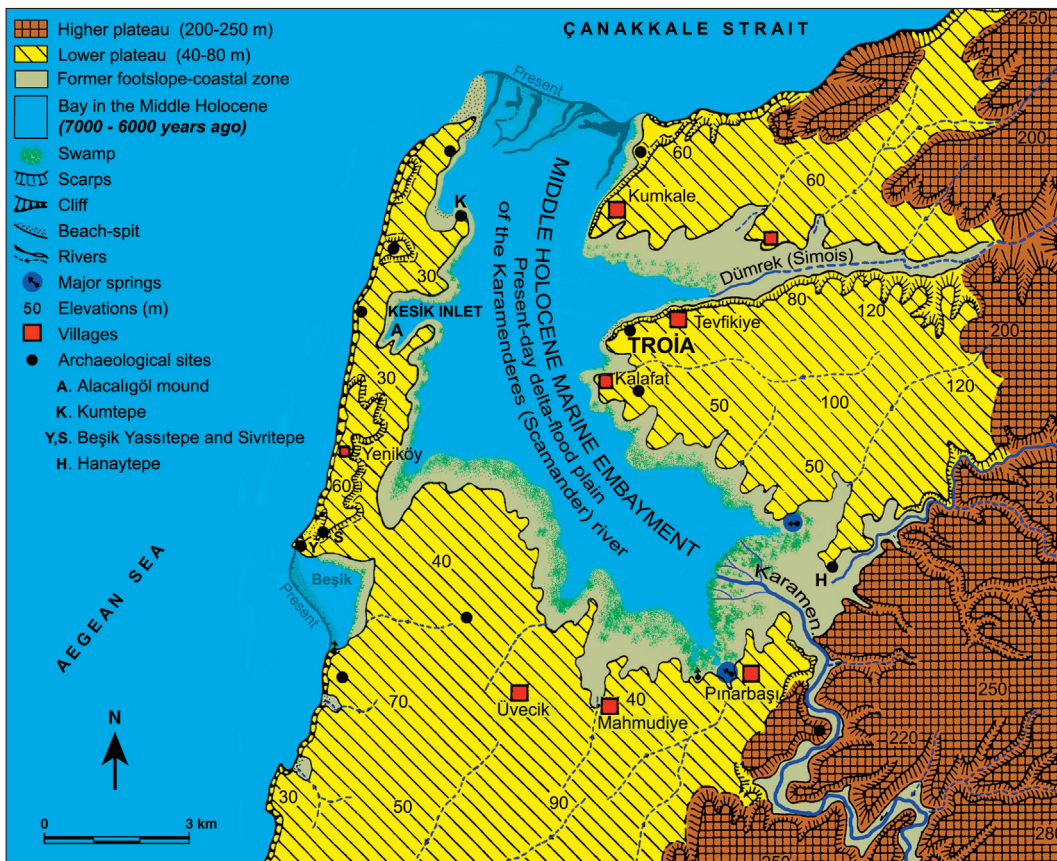
Fig. 4 Paleogeographical reconstruction of the lower parts of the Karamenderes (Sca-mander) and Dümrek (Simois) valleys in the Middle Holocene, about 7000–6000 years ago. In this period, the lower Karamenderes valley was completely covered by the rising sea and formed a marine embayment. A Troia settlement did not exist yet. However, the Alacalıgöl and Kumtepe Neolithic settlements were already established on the shoreline of the embayment.
