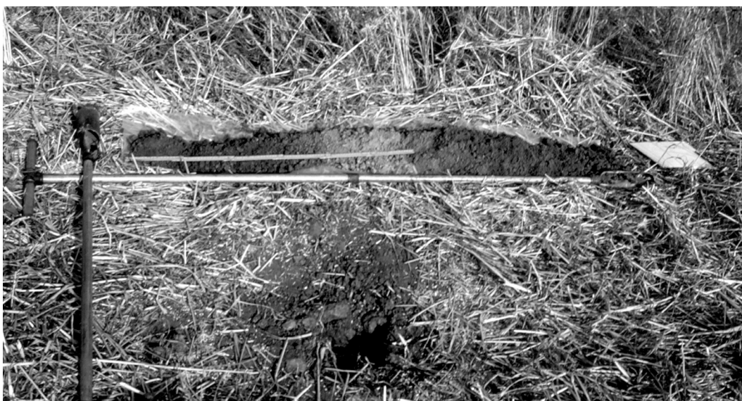
Fig. 5 Sample profile of an Eijkelkamp hand drilling equipment, which was used on the Beşik plain generally. Sinking about 8–10 m deep is possible with this tool. As it is seen on the photograph, sediment samples could not be taken under undisturbed conditions. However, it is possible to separate different recent sediment units and soil horizons. The equipment on the photograph is not original. Corer-ends are handmade by a smith and extension rods are water pipes. Our first studies were performed using this simple tools.
